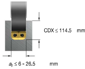
Tailor Made "Vol" groeffrezen met radius
